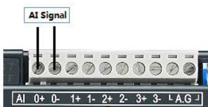
Figure 3.2 Analog Input Wiring
