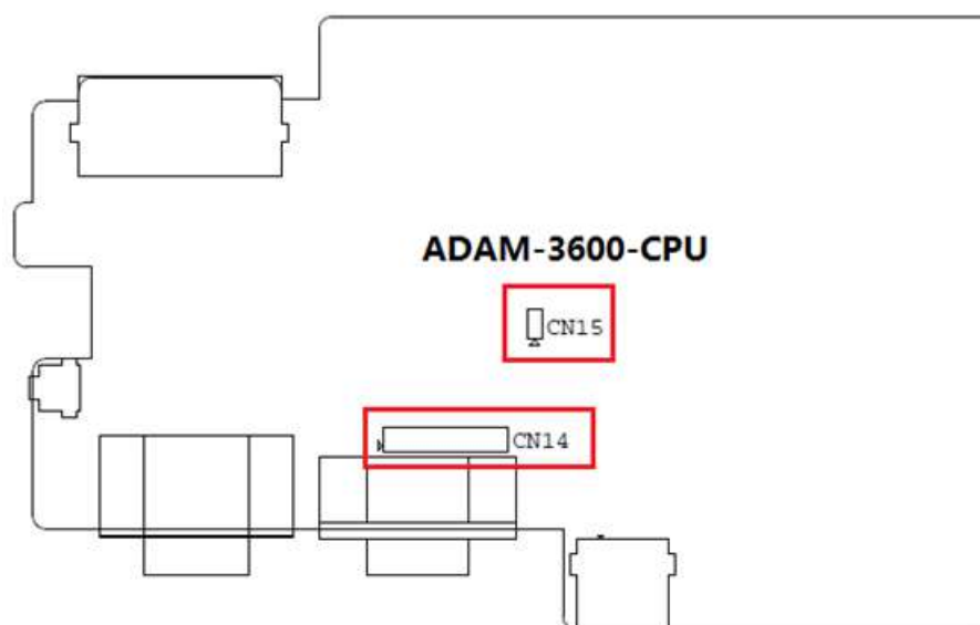
Figure 3.15 Jumper Settings
