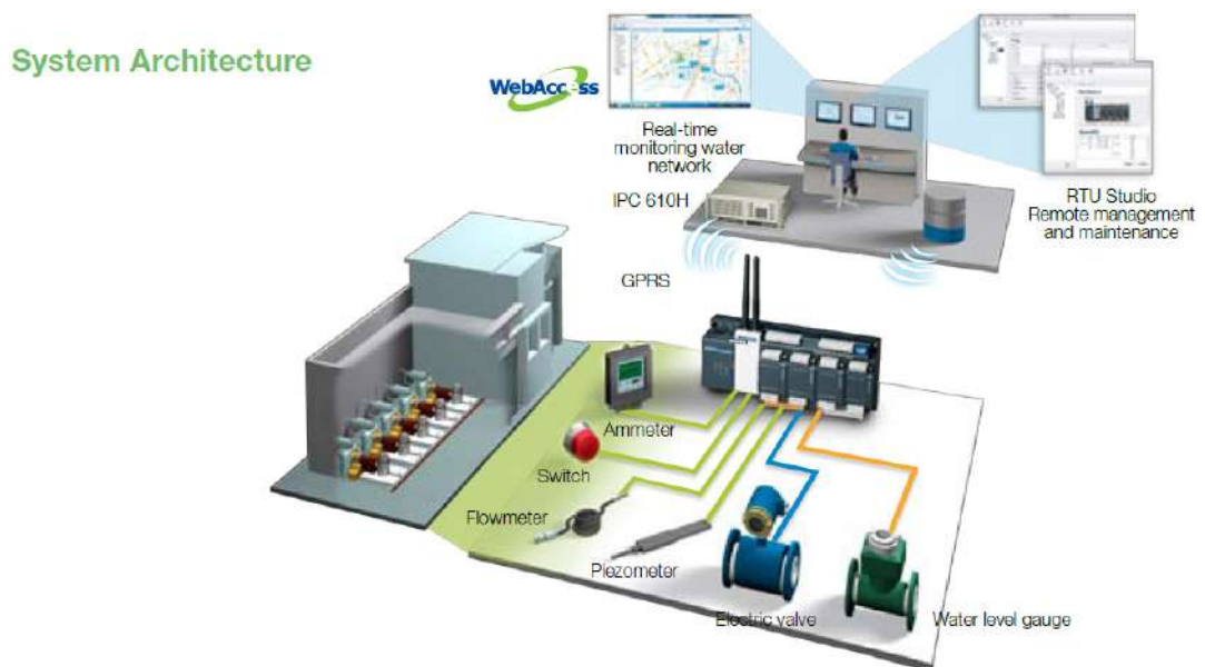
Figure 1.1 iRTU Application Architecture
